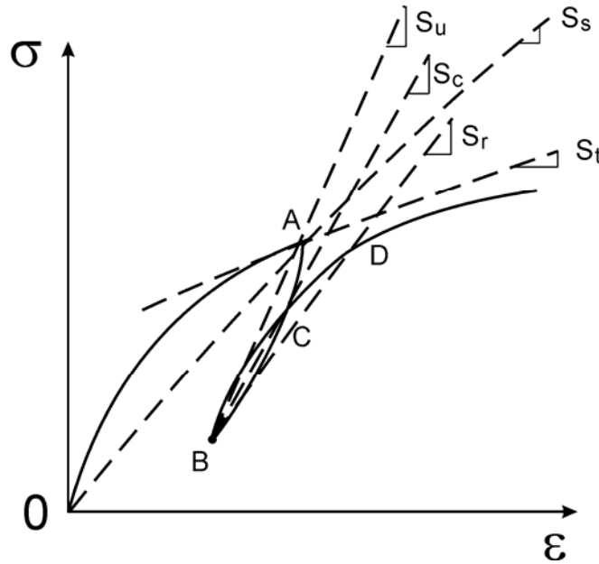
Fig. 2 – Definition of Soil Modulus
