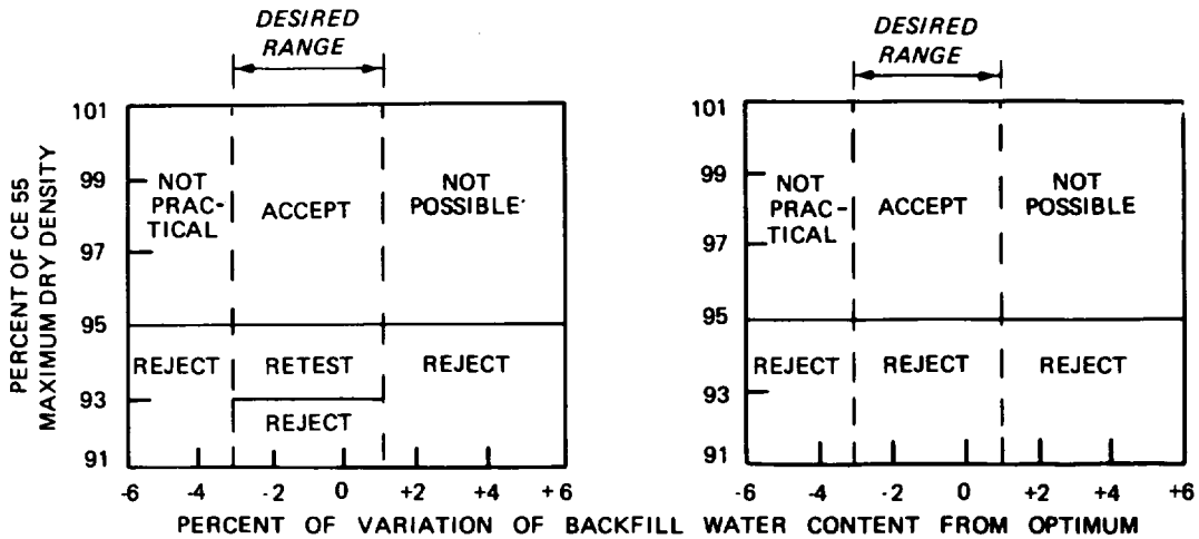
a. USE FOR INITIAL TEST OF BACKFILL AT RANDOM LOCATION
