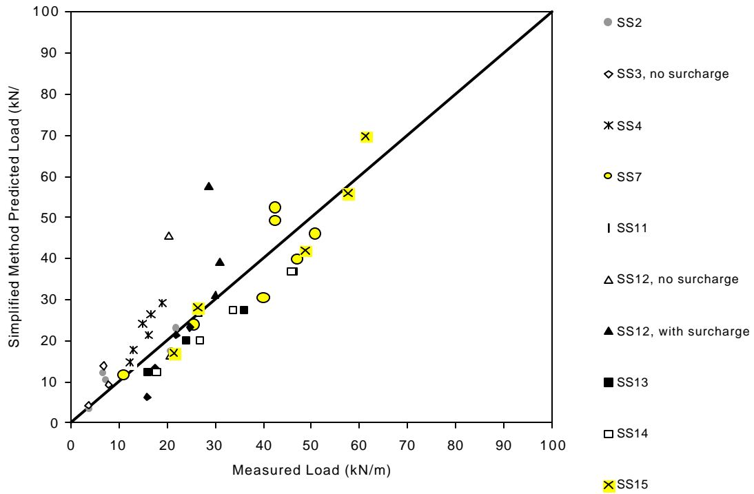
Figure 28. Simplified Method predicted load versus measured reinforcement peak load for steel strip reinforced MSE walls, with \phi greater than 40^\circ .
