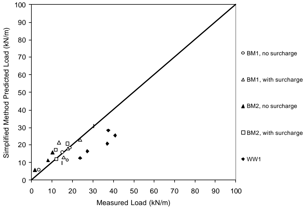
Figure 30. Simplified Method predicted load versus measured reinforcement peak load for steel bar mat and welded wire reinforced MSE walls, with phi greater than 40°.
