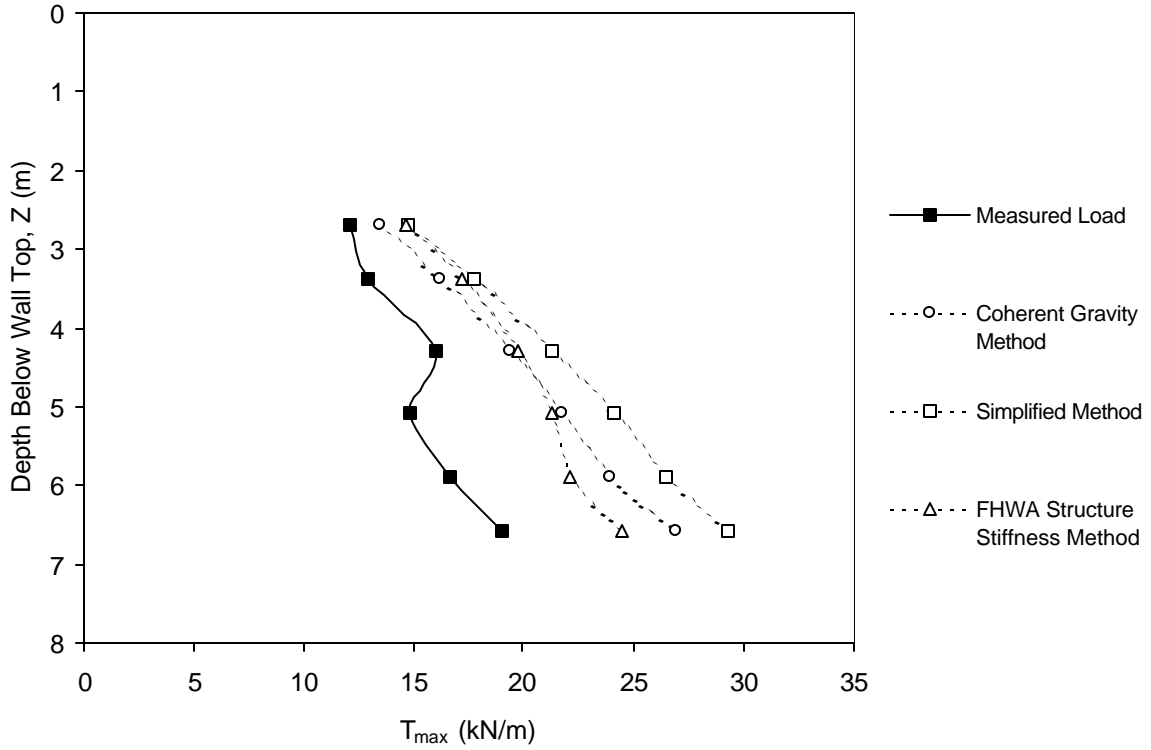
Figure A-7. Predicted and measured reinforcement peak loads for Fremersdorf, Germany, steel strip reinforced wall (SS4).
