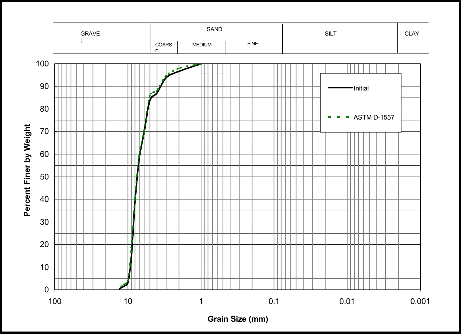
Figure A.4: Initial grain size curve of Ft. Worth soil (SP) and curves after impact compaction tests
