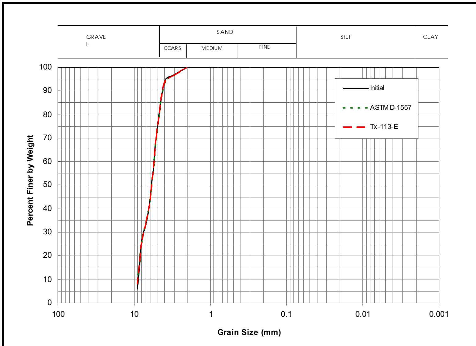
Figure A.12: Initial grain size curve of Acala soil (SP-SM) and curves after impact compaction tests
