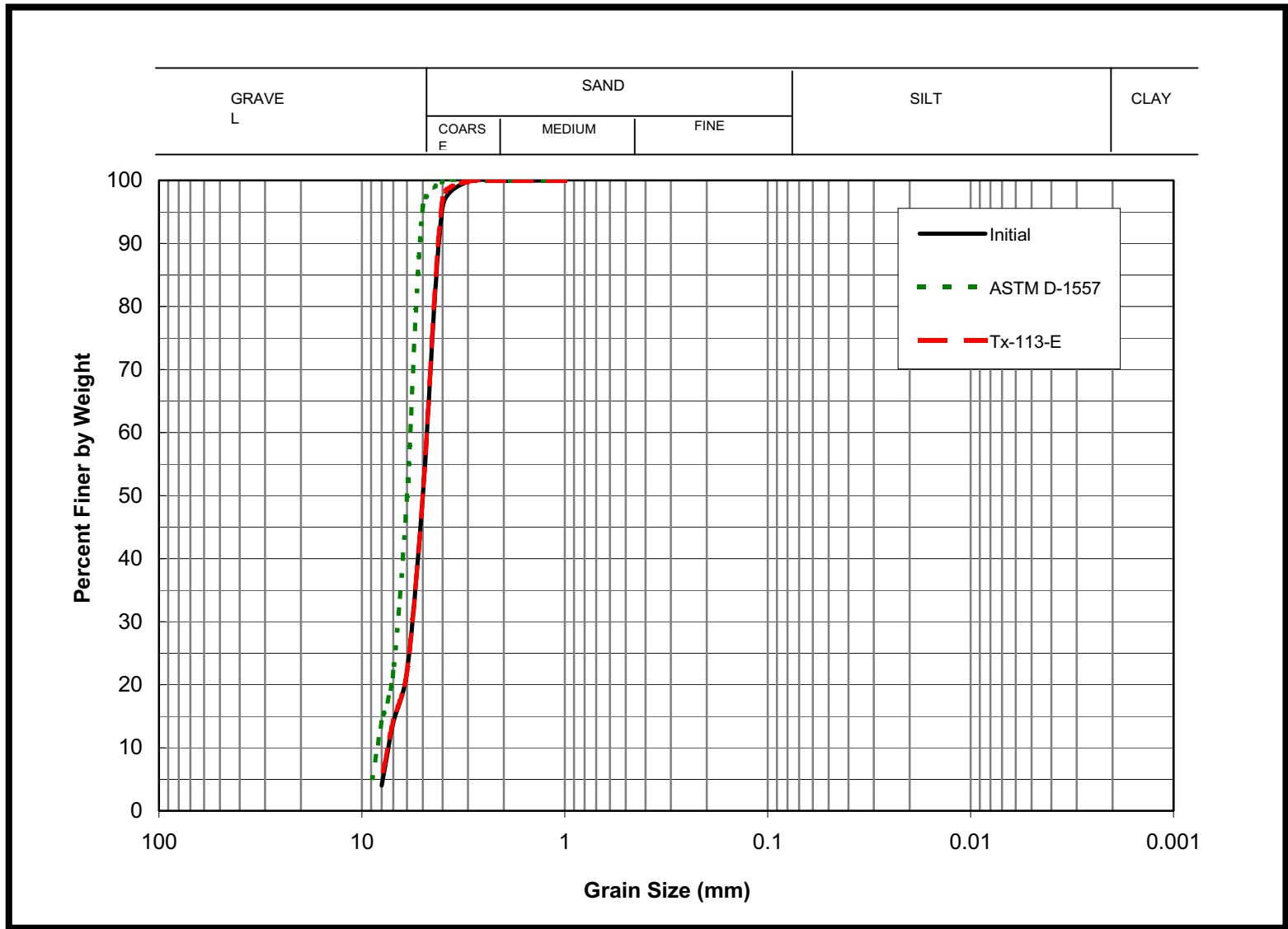
Figure A.2: Initial grain size curve of McNary soil (SP) and curves after impact compaction tests
